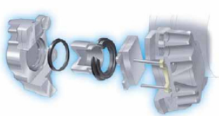
Boot Piston, Boot Pin, Piston Seal
